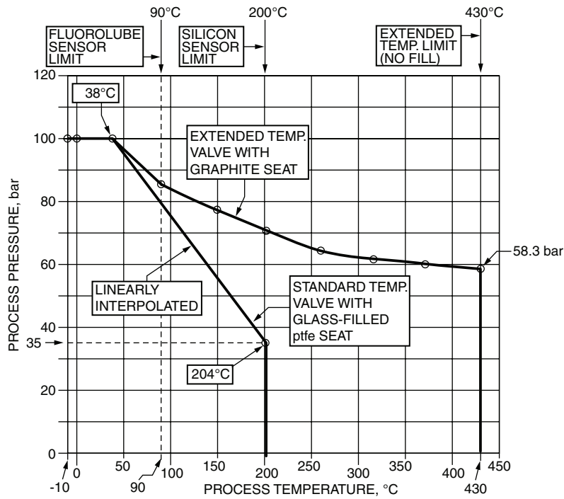
Figure 6. Pressure-Temperature Limits with Isolation Valves
