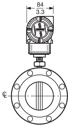
84F (Style B) FLANGED BODY
