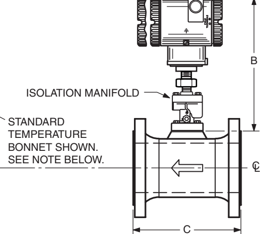
84F (Style B) WITH ISOLATION VALVE
