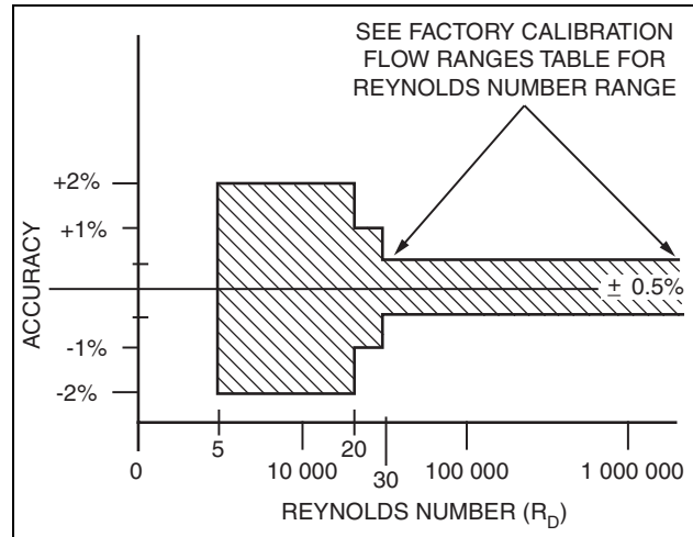
Figure 2. Flowmeter Accuracy for Liquids
