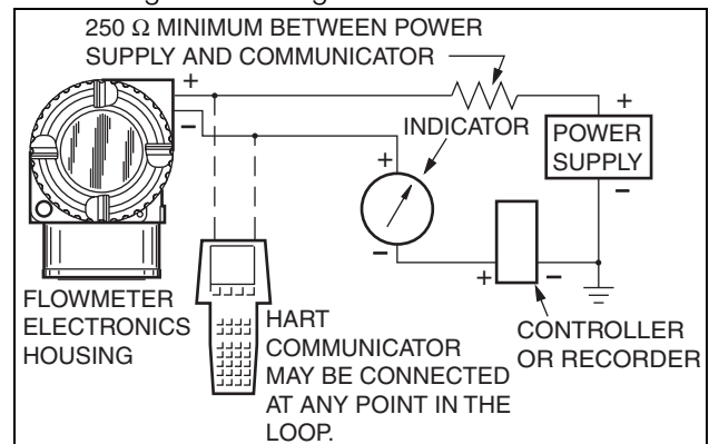
Figure 4. HART 4 to 20 mA Topology
