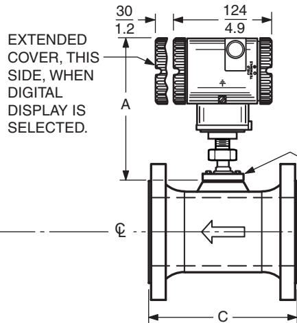
84F (Style B) FLANGED BODY
