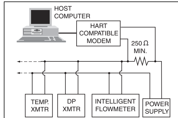
Figure 5. HART Multidrop Topology
