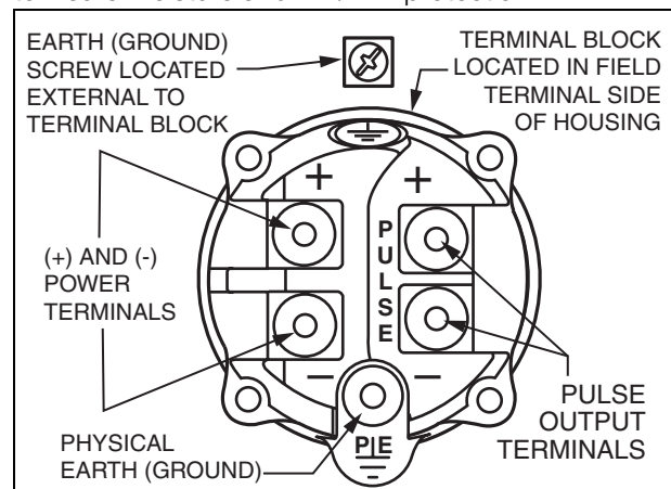
Figure 7. Terminal Block
